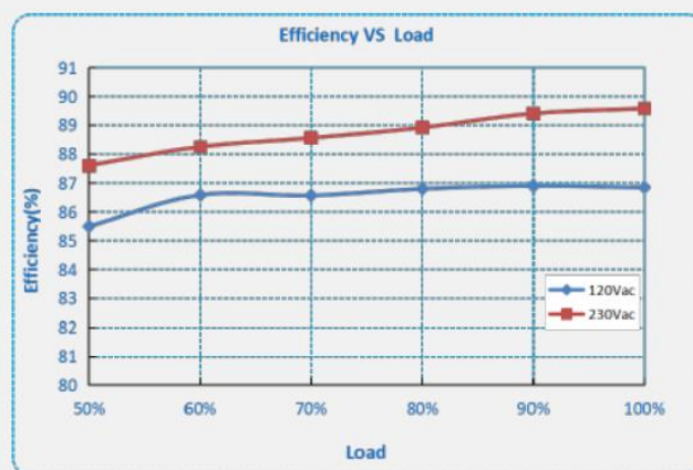
F1-060X-085 ( I_o=0.7A )
